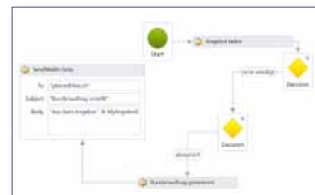
Workflowdesigner
